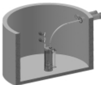
Pit-installed pump
